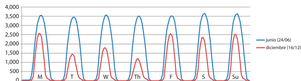
Power (MW) generated by PV solar plants in Spain for the week of June 24-30, 2013, compared to the week of December 16-22, 2013 [REE 2013].
