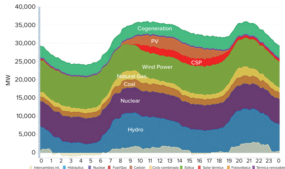
Figure 7.1 Typical daily generation of electricity in Spain from different sources [REE 2013].
