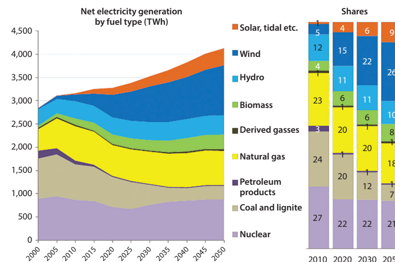
Figure 9.2. Electricity generation (TWh) in Europe by fuel type and projections to 2020, 2030, and 2050 according to the “EU Energy Trends” [EU 2014].
