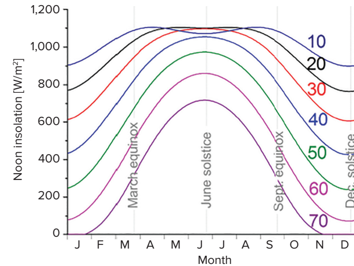
Figure 7.6. Noon solar insolation ( \text{W/m}^2 ) as a function of the month of the year and for latitudes from 10^\circ to 70^\circ in the northern hemisphere.
