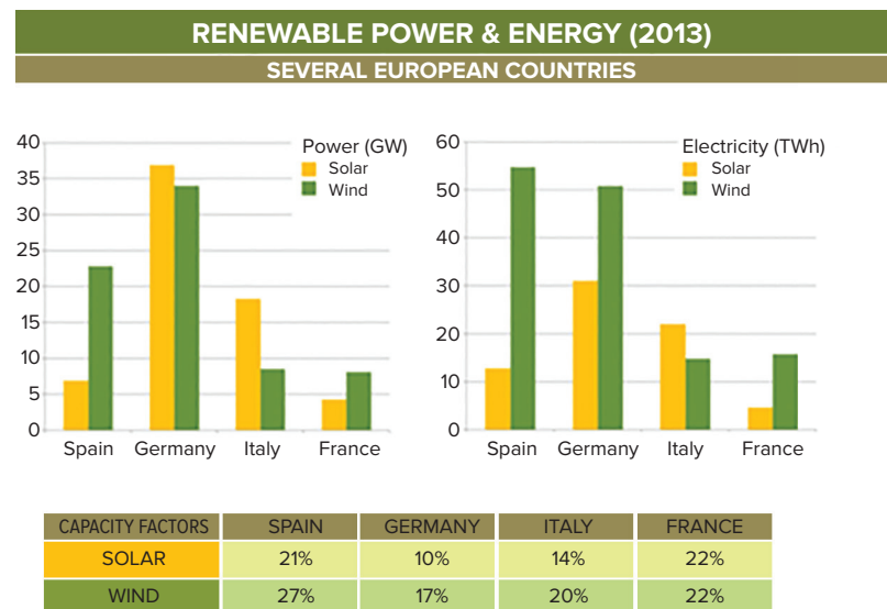
Figure 4.2. Renewable power, energy, and capacity factors in several European countries.
