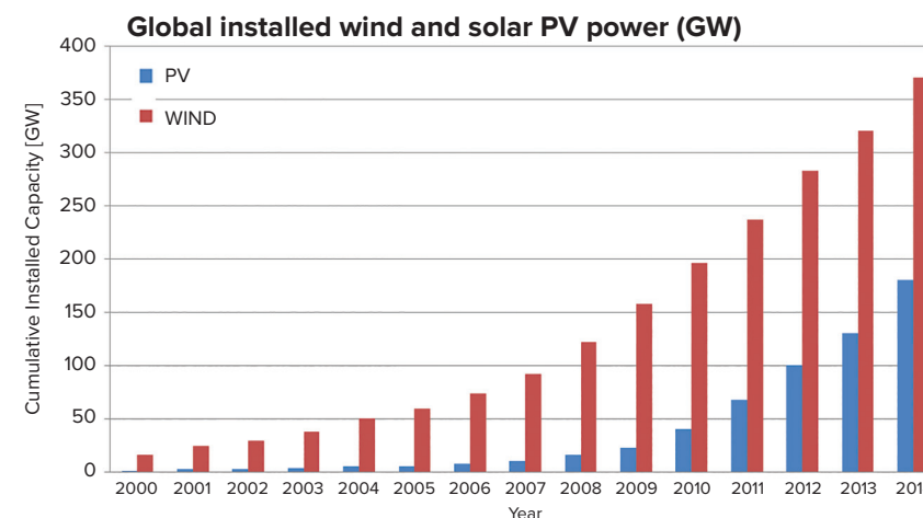
Figure 4.3. Evolution (2000-2014) of the global installed capacity for wind power and solar PV [Jäger-Waldau, A. 2014, REN21 2015, Martinez-Duart, J. et al. 2015].
